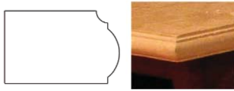
Classic Rail - 1 1/2"
